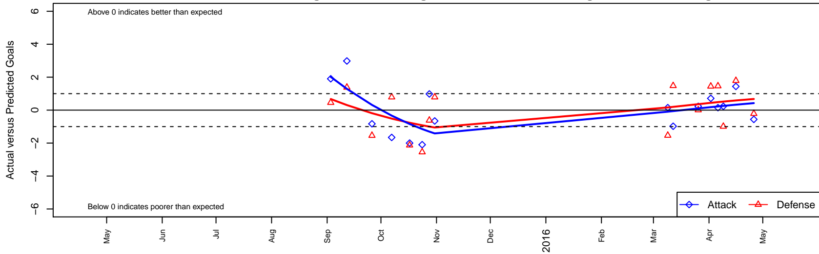
FC Nova Red LR G03 Dots are actual minus expected GF (blue circles) and GA (red triangles). Blue line is smoothed change in attack strength. Red is smoothed change in defense strength.
